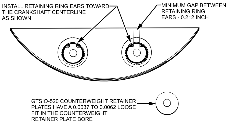
Figure 3. Counterweight Inspection (Applicable to GTSIO-520 Only)
